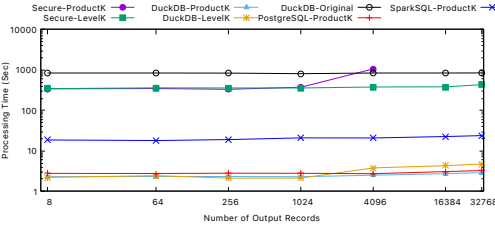
Fig. 6. Running time v.s. different K (Line-3, Twitter).
